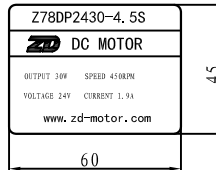
Nameplate
