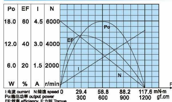
RS-555246000 特性曲线 CHARACTERISTICS
