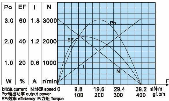
RS-545124500 特性曲线 CHARACTERISTICS
