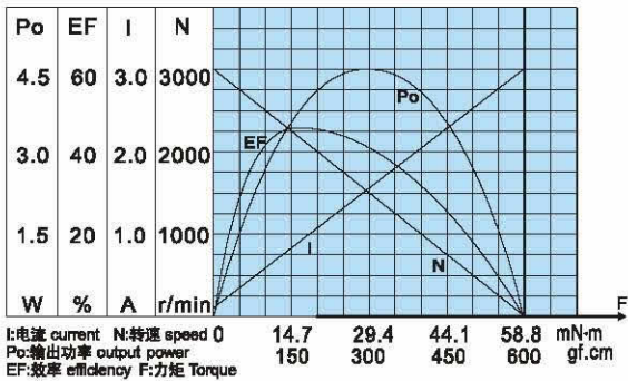
RS-555124500 特性曲线 CHARACTERISTICS
