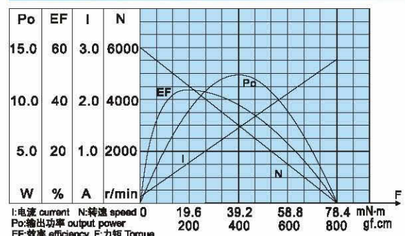
RS-545246000 特性曲线 CHARACTERISTICS
