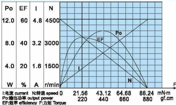
RS-555126000 特性曲线 CHARACTERISTICS
