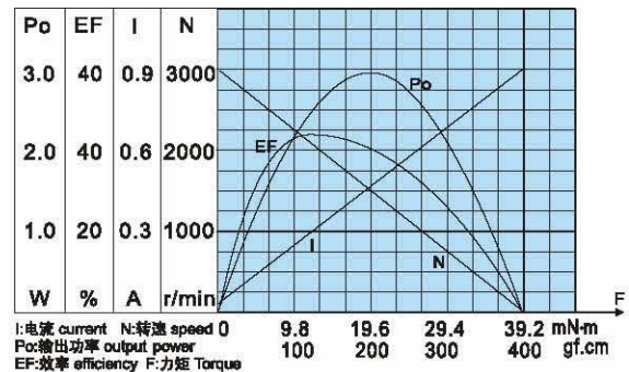
RS-545244500 特性曲线 CHARACTERISTICS
