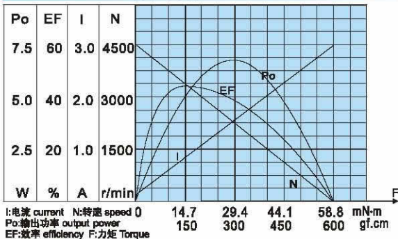
RS-545126000 特性曲线 CHARACTERISTICS
