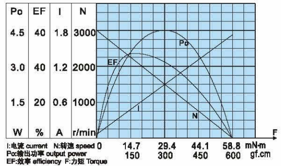
RS-555244500 特性曲线 CHARACTERISTICS
