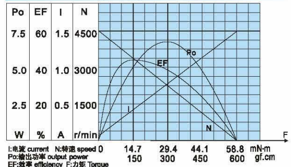
RS-545246000 特性曲线 CHARACTERISTICS
